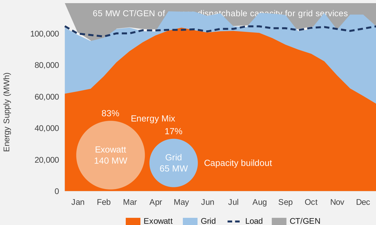
Figure 9. Annual generation profile of the grid-connected configuration
