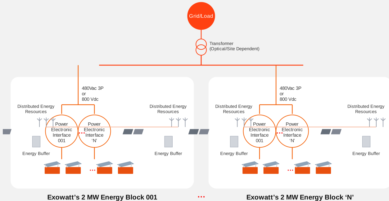
Figure 10. Exowatt's Power System Architecture
