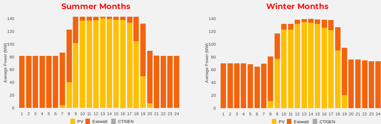
Figure 8. Hourly dispatch of Exowatt, PV, and fuel-based generation
