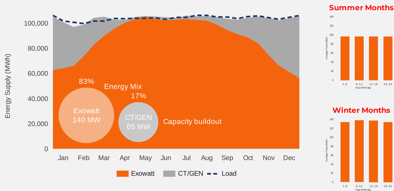
Figure 6. Annual generation and hourly profile of Exowatt and fuel-based generation (off-grid)
